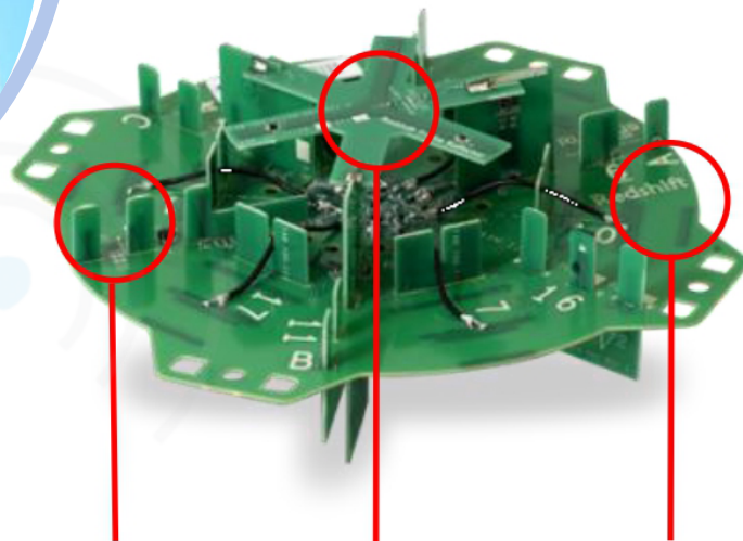
Vertically-polarized antenna elements
