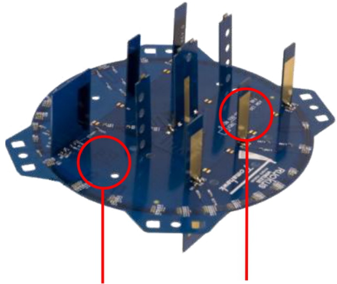
Horizontally-polarized antenna elements
